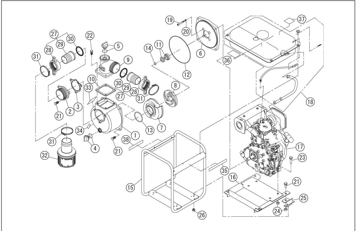
DWG No.012942702 MODELE : SEY-80D FORM : SEY-80D-BAB-0
