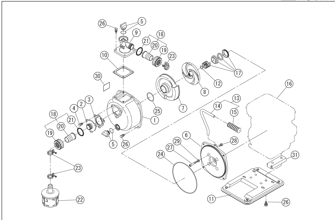
DWG No.012921503 MODELE:SEV-40F FORM:SEV-40F-BAA-0(K100)
